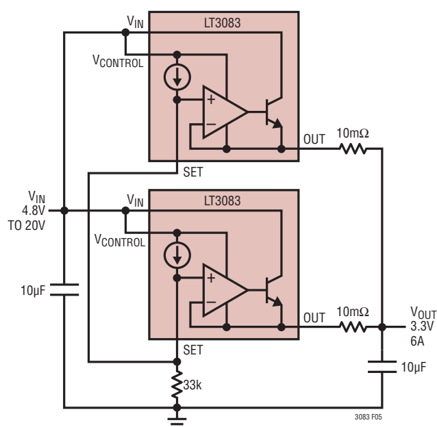
Figure 5. Parallel Devices
